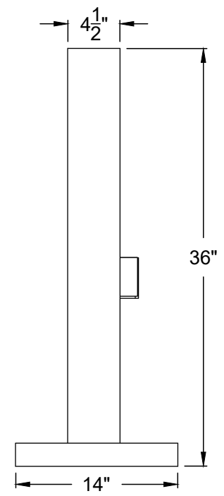
SIDE
